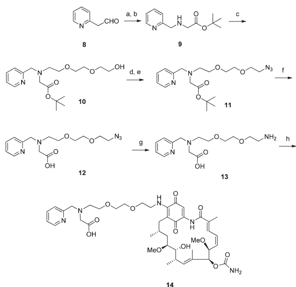
Scheme 3 Reagents and conditions for compound 12 : (a) glycine- tert -butyl ester, toluene, reflux, 2 h; (b) NaBH 4 , MeOH, r.t., 1 h; (c) 2-(2-(2-iodoethoxy)ethoxy)ethanol, NaCO 3 , acetone–water, reflux, 5 h; (d) MsCl, TEA, THF, 0 °C to r.t., overnight; (e) NaN 3 , CH 3 CN, reflux, 4 h; (f) TFA, CH 2 Cl 2 , r.t., overnight; (g) 10% Pd/C, 1.8 bar H 2 , MeOH, r.t., 2 h; (h) GA, compound 13 , DMSO, r.t., 4 h.
